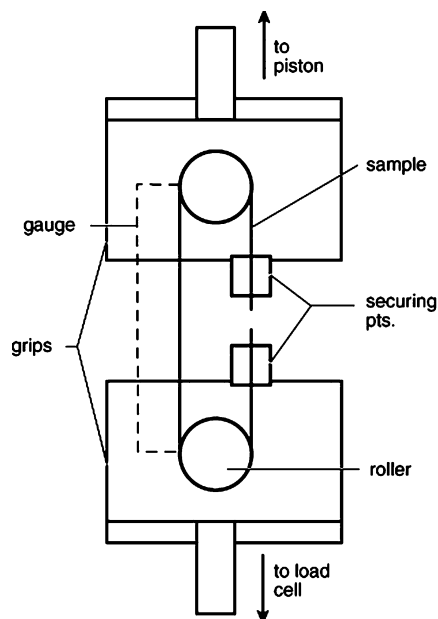
Fig. 1 Roller grips designed for the testing of implant materials
