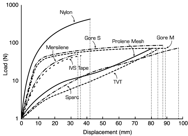
Fig. 4 Typical load-deformation curves for the eight tested permanent materials (log scale). The vertical dotted lines indicate the displacement at which failure occurred
